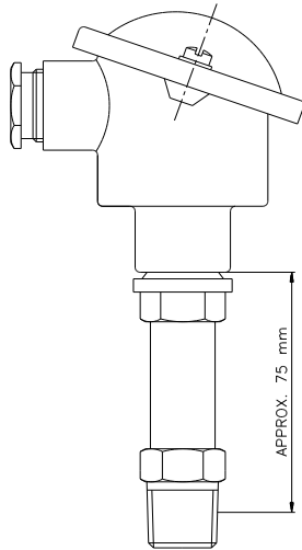
Cast aluminium head
